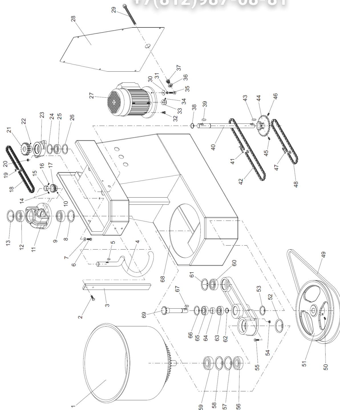
Fig. 7.3. GALASSIA 18-25-35-45-60 - Components of trasmission unit
