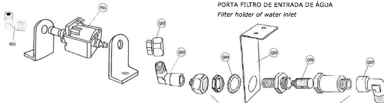
BLOCO DISTRIBUIDOR Distribution unit
